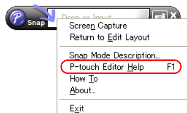
Snap Mode
