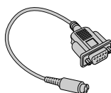
DIN-D-sub RS-232C adaptor (5 57 / 64 " (15 cm)) QCNWGA015WJPZ
