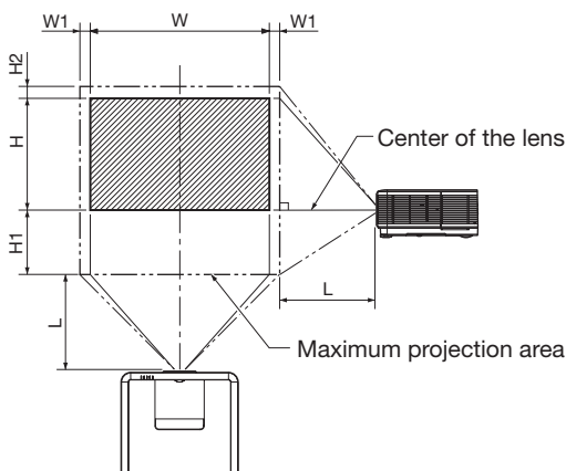
Front projection
