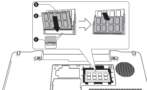
Figure 3-12 Seating the memory module
