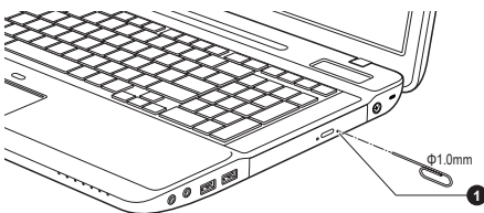
Figure 3-7 Manual release with the eject hole
