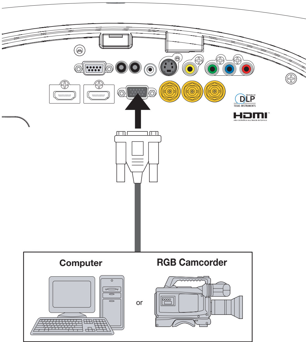
Figure 3-9. RGBHV Connections
