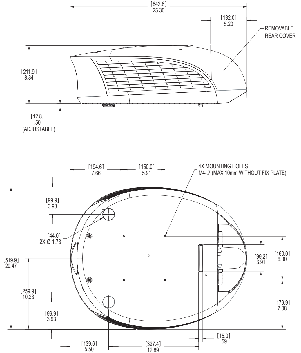
Figure 7-1. LS-10i Dimensions
