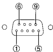
D-SUB 9-pin connector seen from outside
