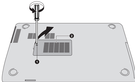
Figure 4-6 Removing the memory module cover
