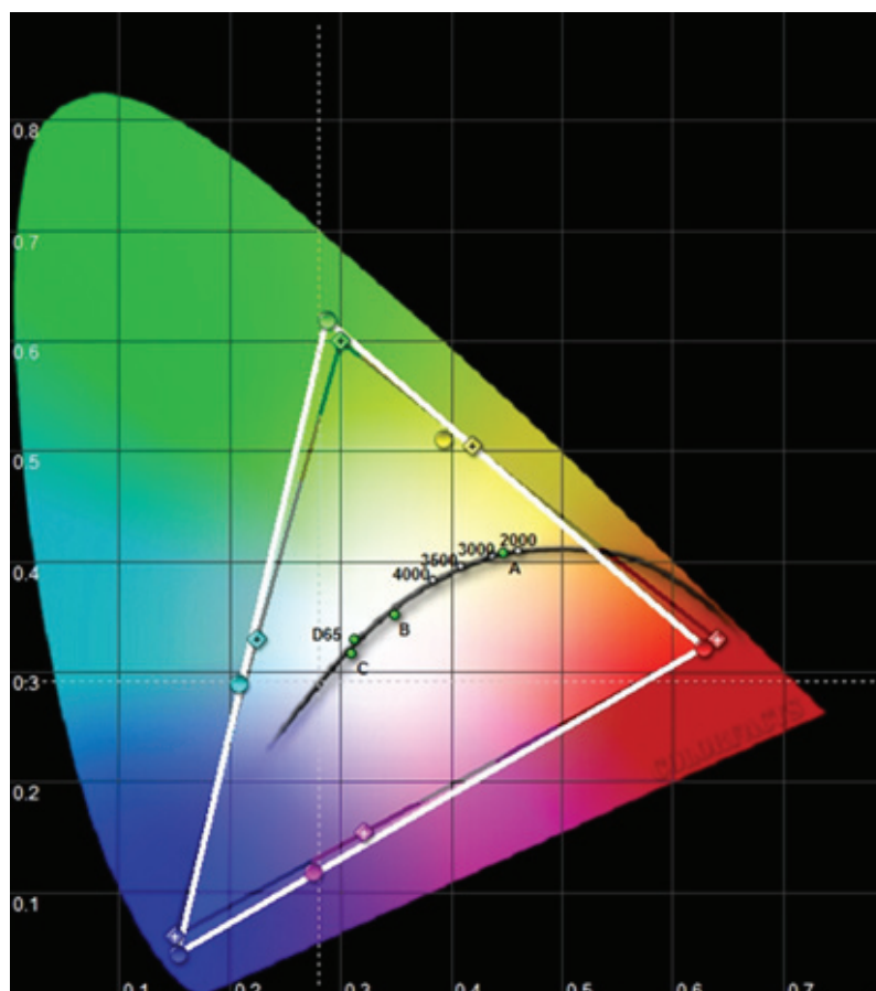
Figure 7-7. CIE Chart with the black body
