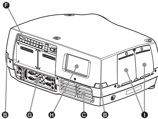
Figure 3-2. - Projector rear view
